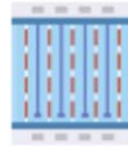
lane line
