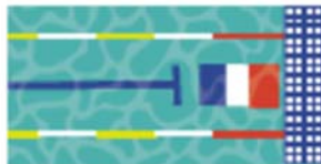
lane
